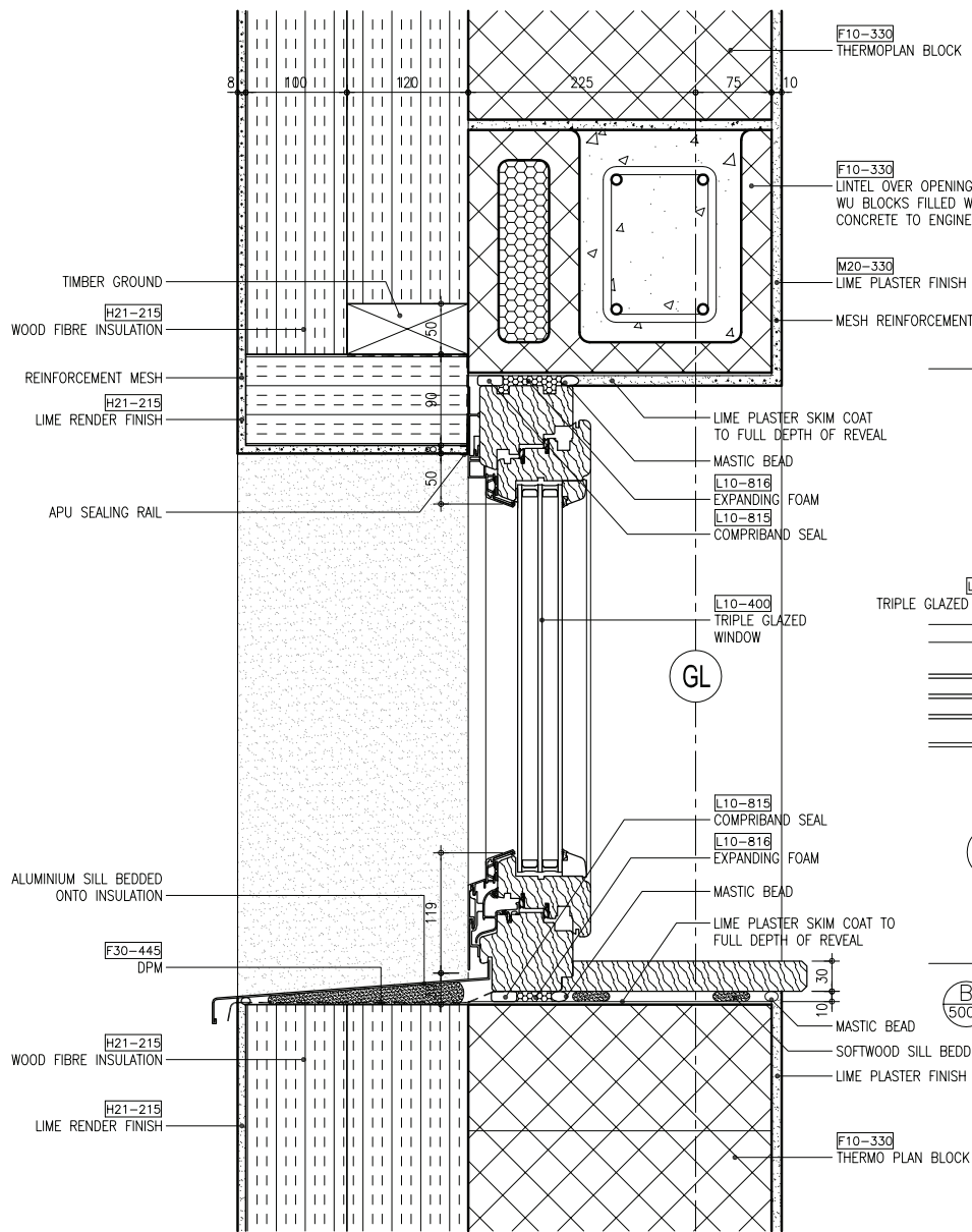
(A) SILL/HEAD SECTION 5004 1:5
